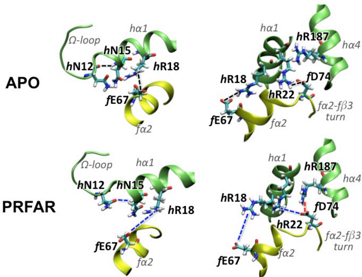
Figure S5. Representative configurations extracted from the MD simulations of the apo (top panels) and PRFAR bound (bottom panels) IGPS complexes, showing the hR18 - fE67 salt-bridge disruption and the resulting partial unfolding of h\alpha1 helix (propagating towards the active site via the \Omega -loop) and rearrangement of interactions between polar/charged residues in h\alpha1 and h\alpha4 helices and the f\alpha2 - f\beta3 turn.
