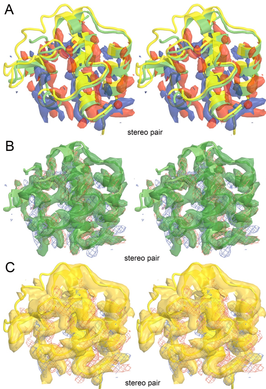
Figure S1. Comparison of a CP43 domain between the Synechocystis 6803 and T. elongatus apo-PSII, in stereodiagram. (A) Vector-difference Fourier map contoured at +12 \sigma (blue) and -12 \sigma (red) superimposed onto the 6wj6 and 6nho coordinates. (B) Experimental map for 6wj6 contoured at +6 \sigma . (C) Experimental map for 7nho contoured at +6 \sigma .
