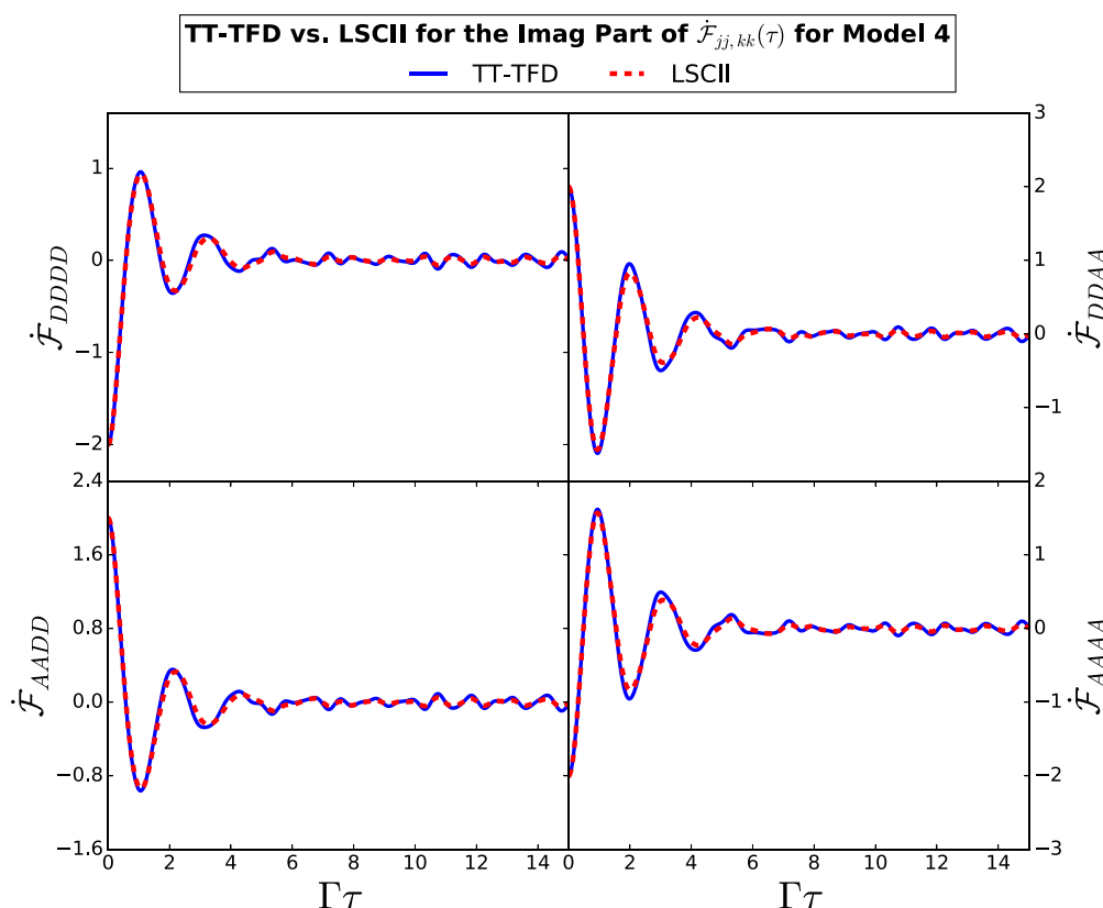
Figure 10. Imaginary parts of the DDDD, DDAA, AADD, and AAAA matrix elements of \tilde{\mathcal{F}}(\tau) (see eq 12) for model 4, as obtained via TT-TFD (solid blue lines) and LSCII (dashed red lines). Similar graphs for the other four models are included in the SI.
