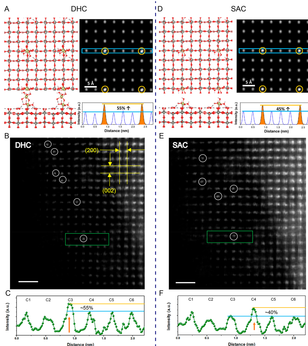
Figure 3. HAADF-STEM studies of end-on bound Ir DHCs on \text{WO}_3 . (A) Atomic structure of Ir DHCs on top of \text{WO}_3 (020). Top left: top view; bottom left: side view. Simulated STEM image from the top view (top right), as well as a representative line scan profile of one Ir DHC against the \text{WO}_3 supporting substrate (bottom right). The positions of the Ir DHCs are marked by orange circles in the simulated STEM image, and the orange-shaded peaks indicate the position of Ir DHCs. (B) Experimental STEM image, in which the region for the line scan profile is marked by the green box. The white circles highlight Ir DHCs. (C) Line scan profile of the region highlighted in (B). (D) Simulated atomic structure of Ir SACs on top of \text{WO}_3 (020). The arrangement of the panels is identical to (A). (E) Experimental STEM image, in which Ir SACs are highlighted by the white circles. The green box marks the region where the line scan profile in (F) was obtained. (F) Line scan profile of the region shown in (E). Scale bars for (B) and (E): 1 nm.
